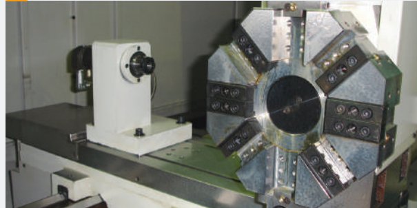
14 Hydraulic 8-Station Turret (Taiwan)
